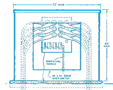
Subsurface Switch with Optional Padmount Enclosure
