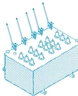
SG6 switch with top mounted spread version bushing arrangement.
