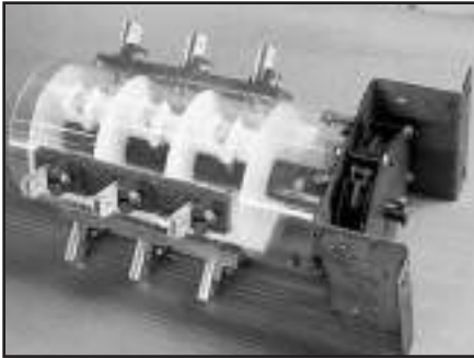
p Three position rotary puffer mechanism.
