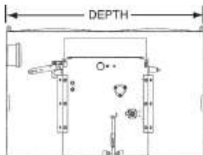
SIDE Source side operating compartment
