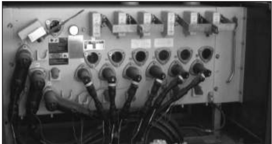
p Model PVI-7F with three phase operating handle.
