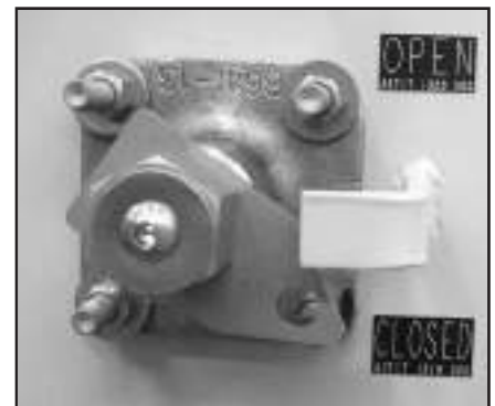
p Load break rotary operator.
