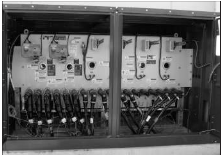
p Padmount switch with SEL controls.
