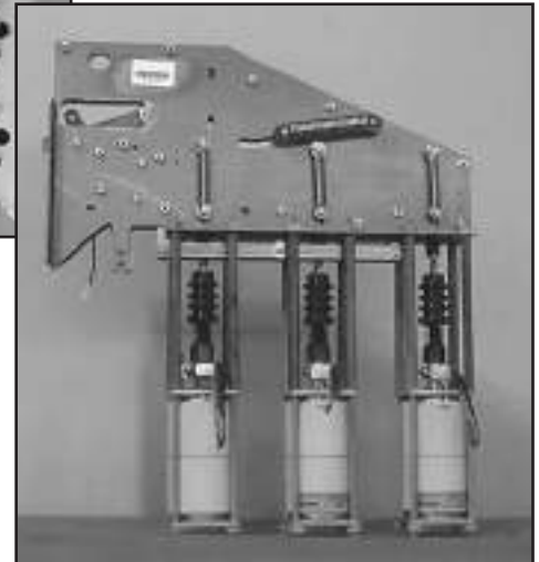
t Three phase interrupter operating handle for manual three phase operation and reset.
