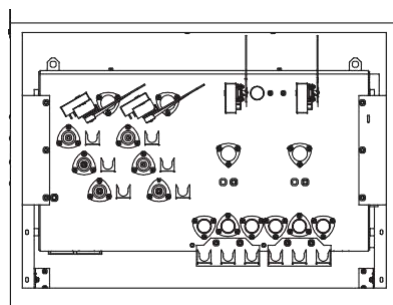
p Load break switch visible break.
